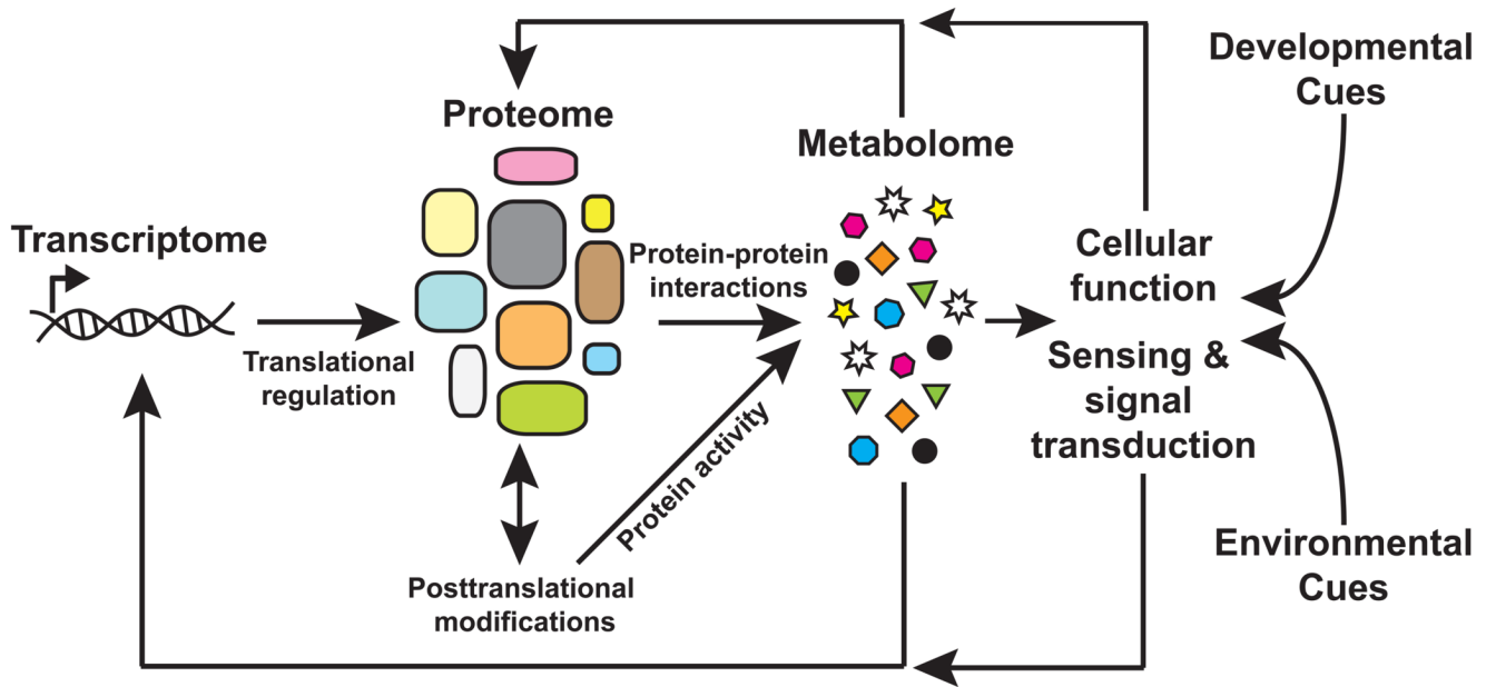
Figure 2. Schematic of a network showing interdependence of system components and response to feedback based on developmental or environmental cues. The metabolic profile of a cell or system provides a measure of the output of the genetic network but may also serve as an input. In response to external cues metabolites feed back into networks, ultimately altering behavior of the system. Figure adapted from Weckworth [23].
